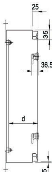
Mounting plate
