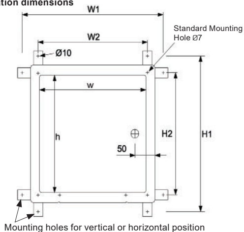
Installation dimensions
