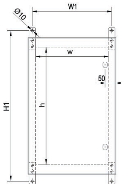
Installation dimensions
