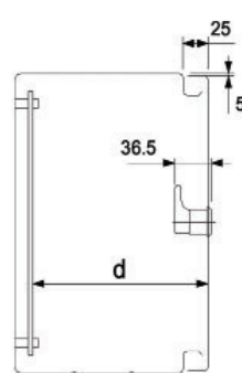
Mounting plate
