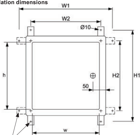
Installation dimensions
