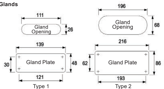
Glands
